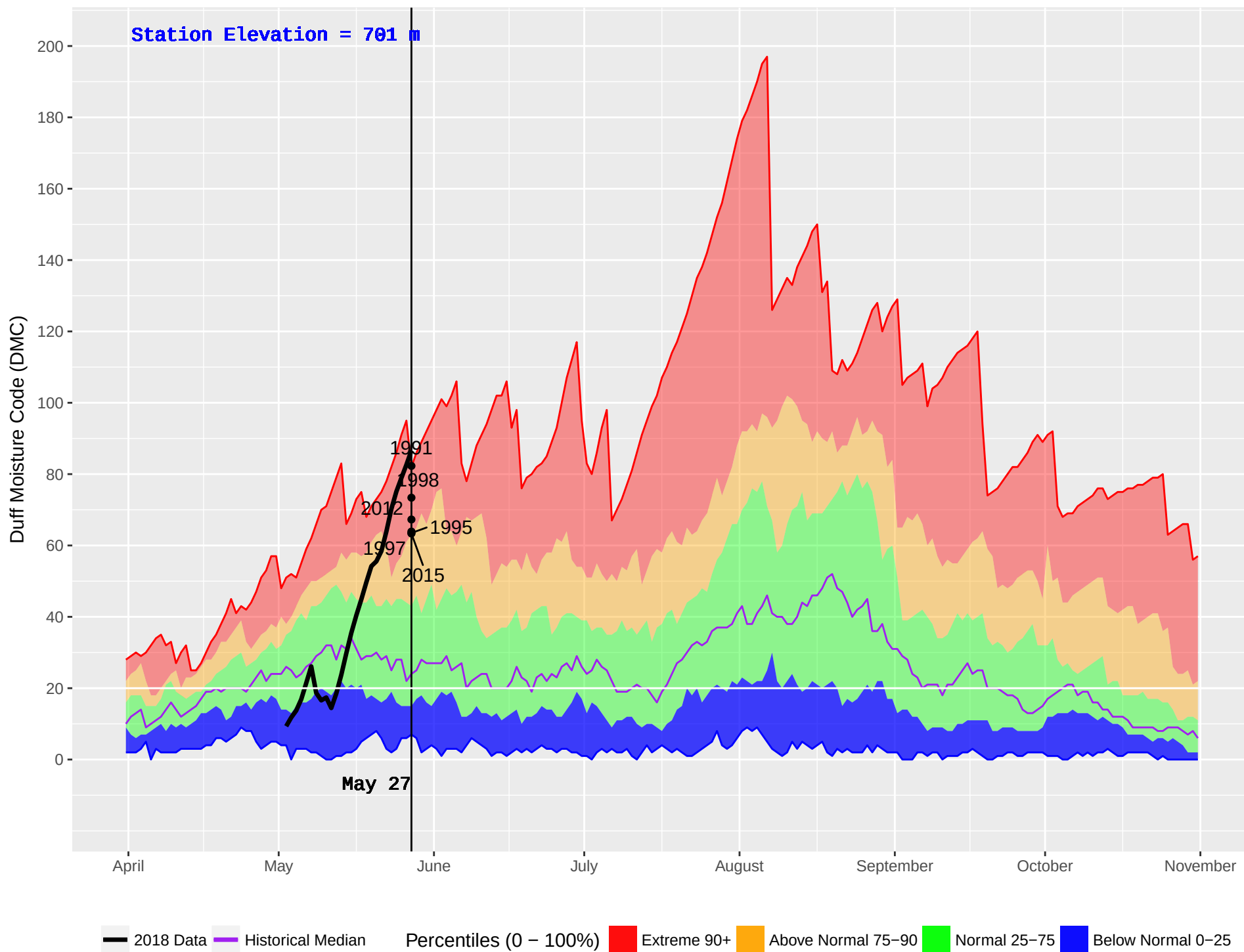
HORSEFLY (230) : Historical (1971–2016) and Current (2018) Noon Duff Moisture Code (DMC)
