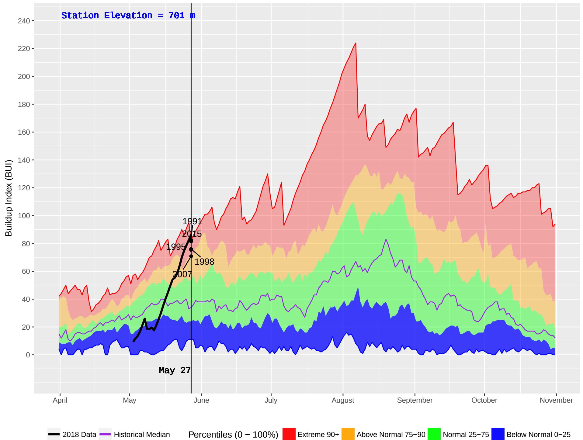
HORSEFLY (230) : Historical (1971–2016) and Current (2018) Noon Buildup Index (BUI)
