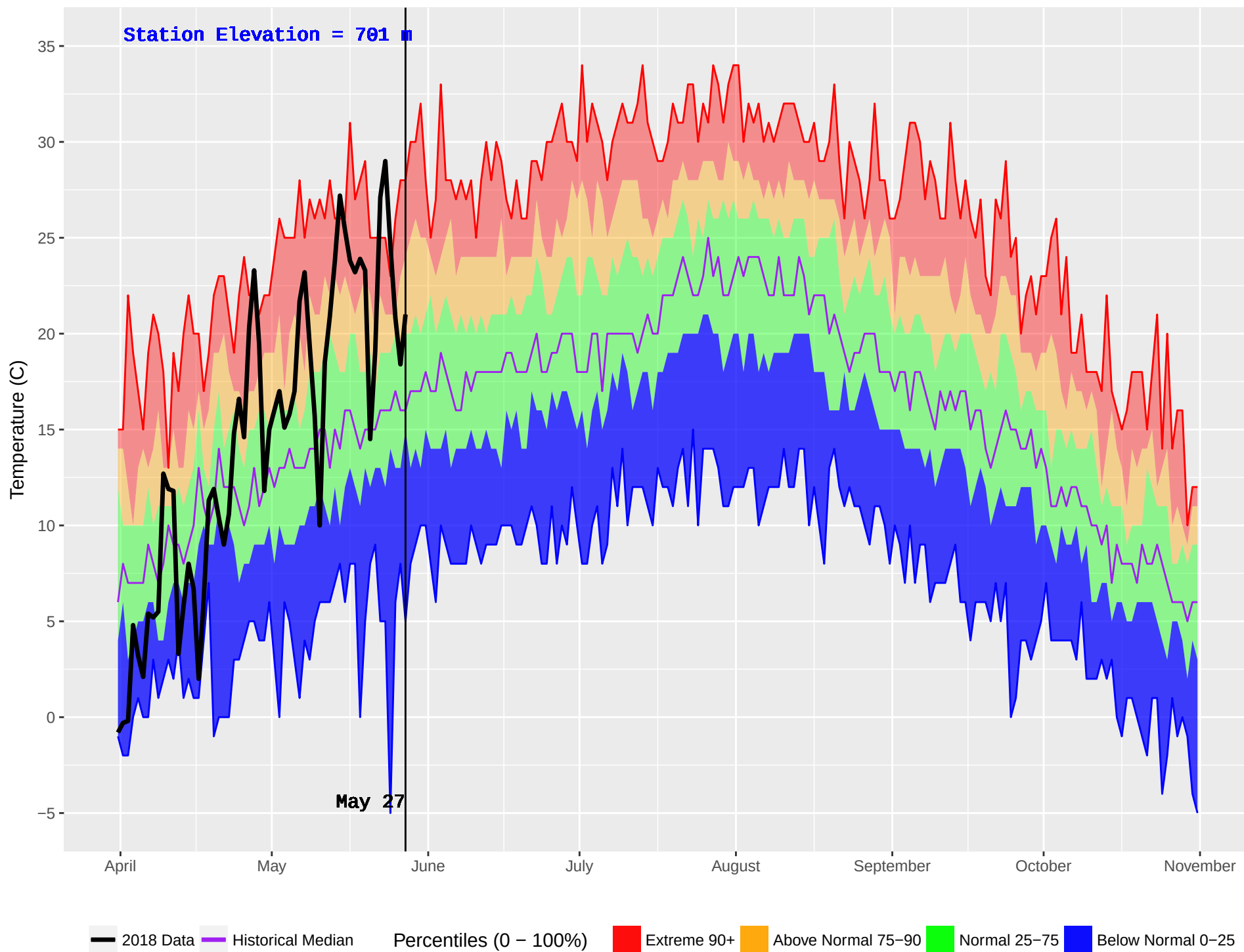
HORSEFLY (230) : Historical (1971–2016) and Current (2018) Noon Temperature
